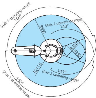
Working Envelope of TH650A
